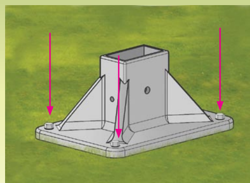
ST10 For attachment to a flat hard ground
