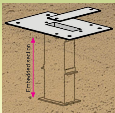
ST09 Specially designed for embedding in the ground
